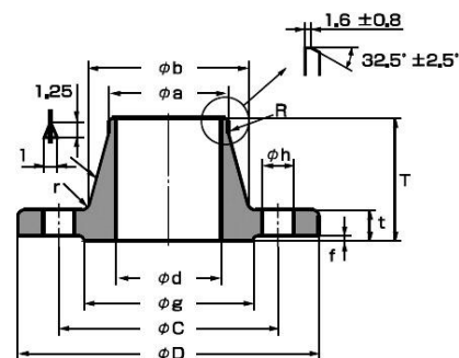
Weld Neck
