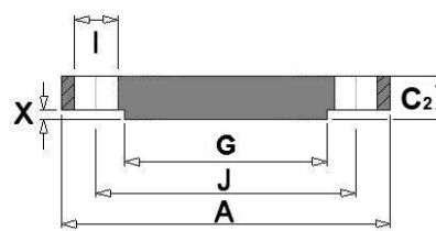
blind
