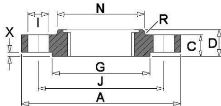
Socket weld
