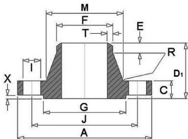
Weld neck
