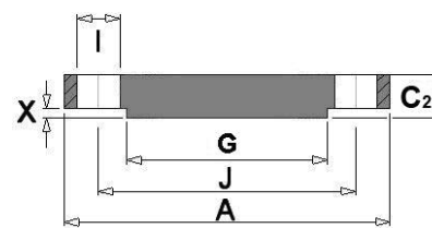
Blind
