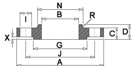
Slip on
