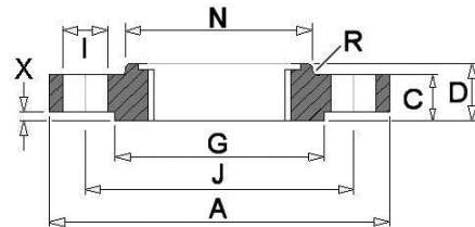
Socket weld
