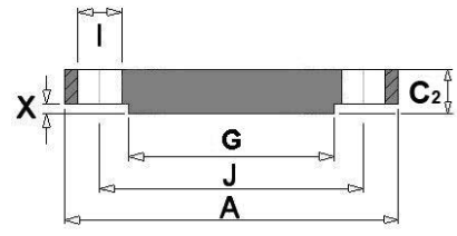
Blind
