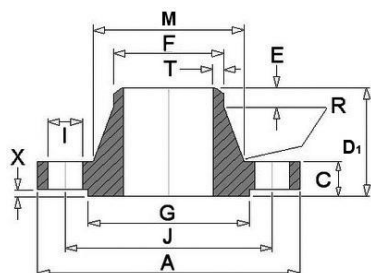
Weld neck
