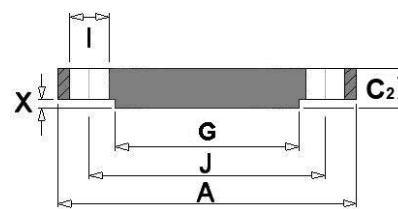
Blind
