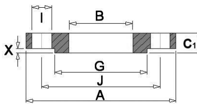
Lap joint
